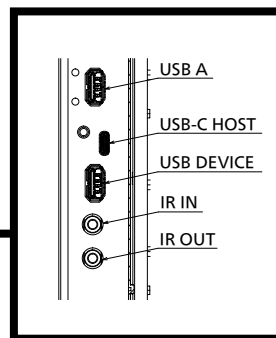
Magnified figure of terminal a
